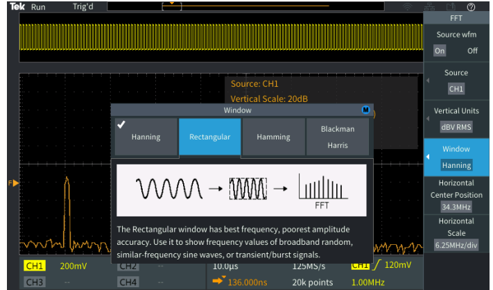
Figure 11: HelpEverywhere tips explain important settings.
