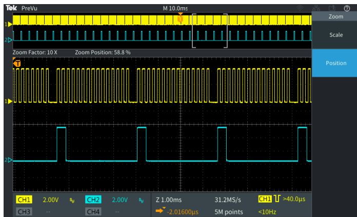
Figure 1: In Zoom mode, an overview of the entire record is shown in the upper part of the display and the lower part displays the detailed Zoomed view.
