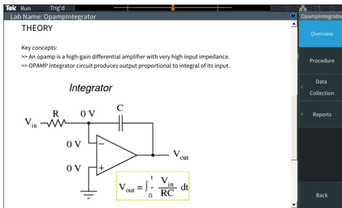
Figure 14: The Courseware function allows students to see lab information on the instrument display.
