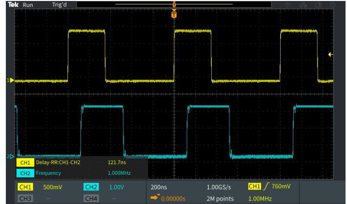
Figure 7: Measurements are transparent so waveforms are not obscured.
